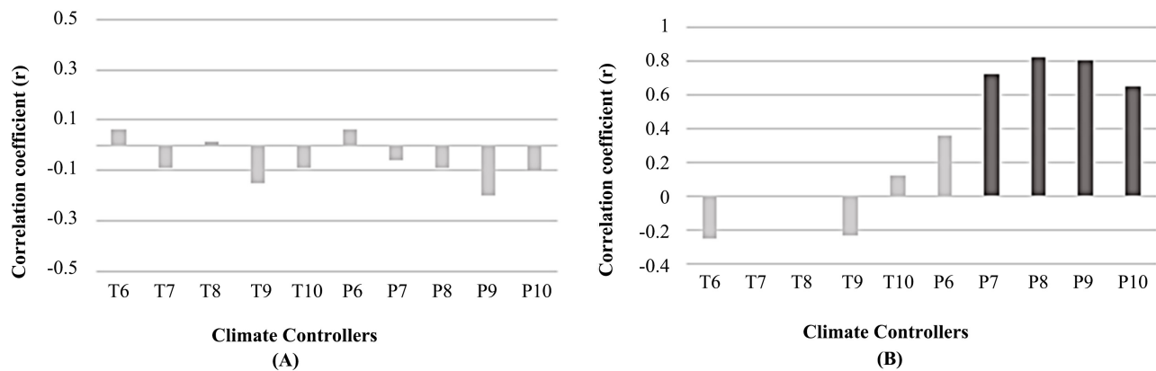
Figure 10. Bootstrap correlation coefficient between the growth chronologies of B. senegalensis (A) and S. Birrea (B) and climate. T: temperature, P: precipitation.
