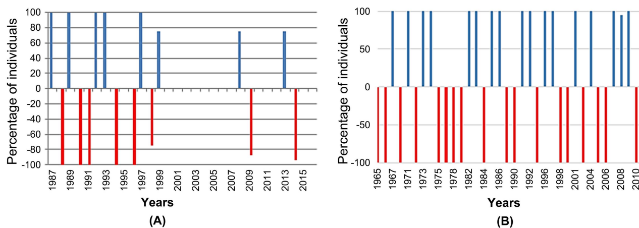
Figure 9. Characteristic years from 1964 to 2016 according to Merian's Pointer Year method (2010) for (A) B. Senegalensis , and (B) S. Birrea (positive characteristic years are in blue and negative characteristic years in red).
