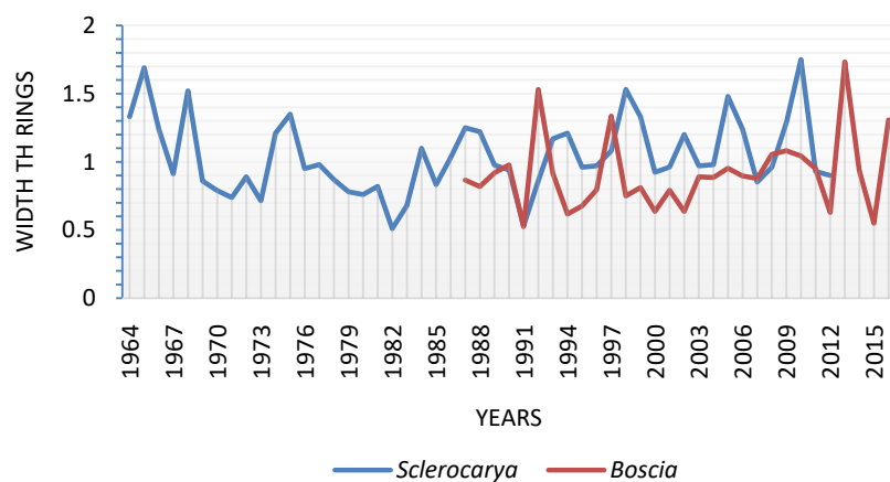
Figure 8. Standardized reference chronologies.
