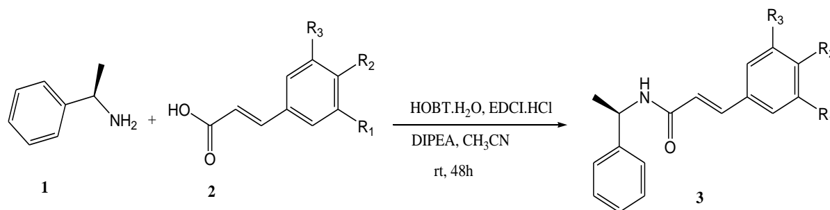
Figure 1: Synthesis of compound 3 acid cinnamic derivatives.
