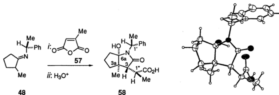
X-Ray crystal structure of 58
